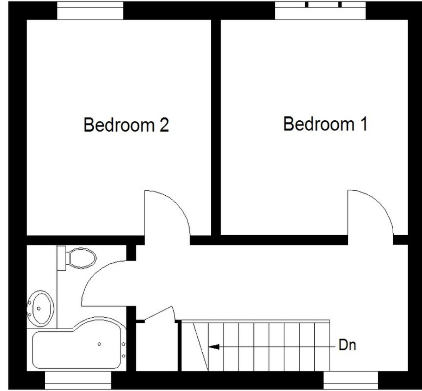
First Floor
